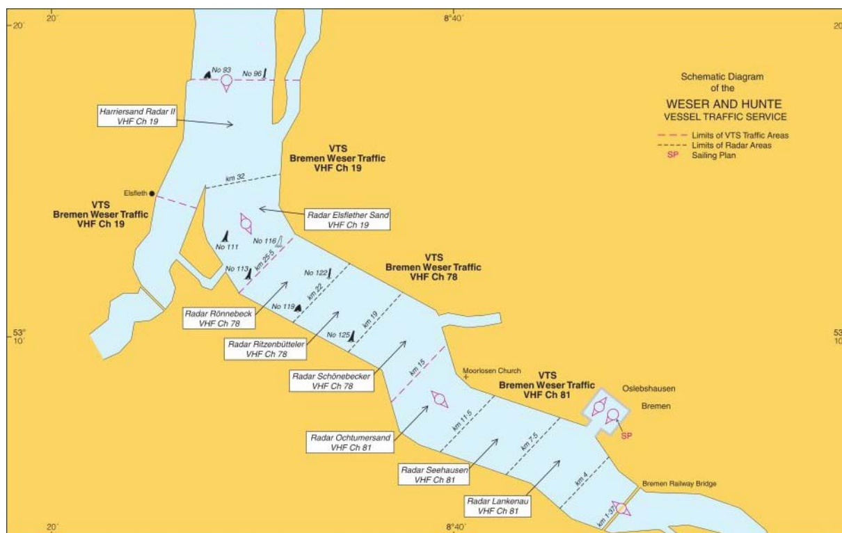
Weser and Hunte VTS (Part 2 of 3)
