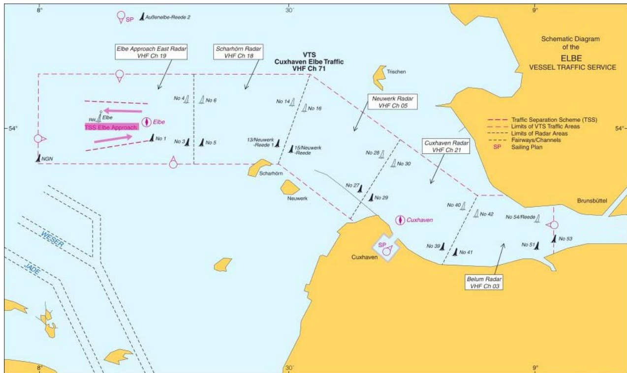
Elbe Western Entrance VTS
