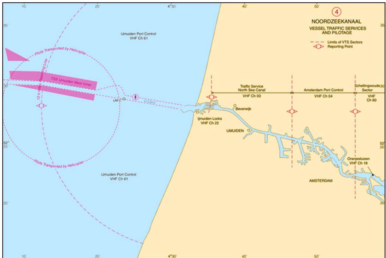
Noordzeekanaal VTS Boundaries and Pilot Stations
