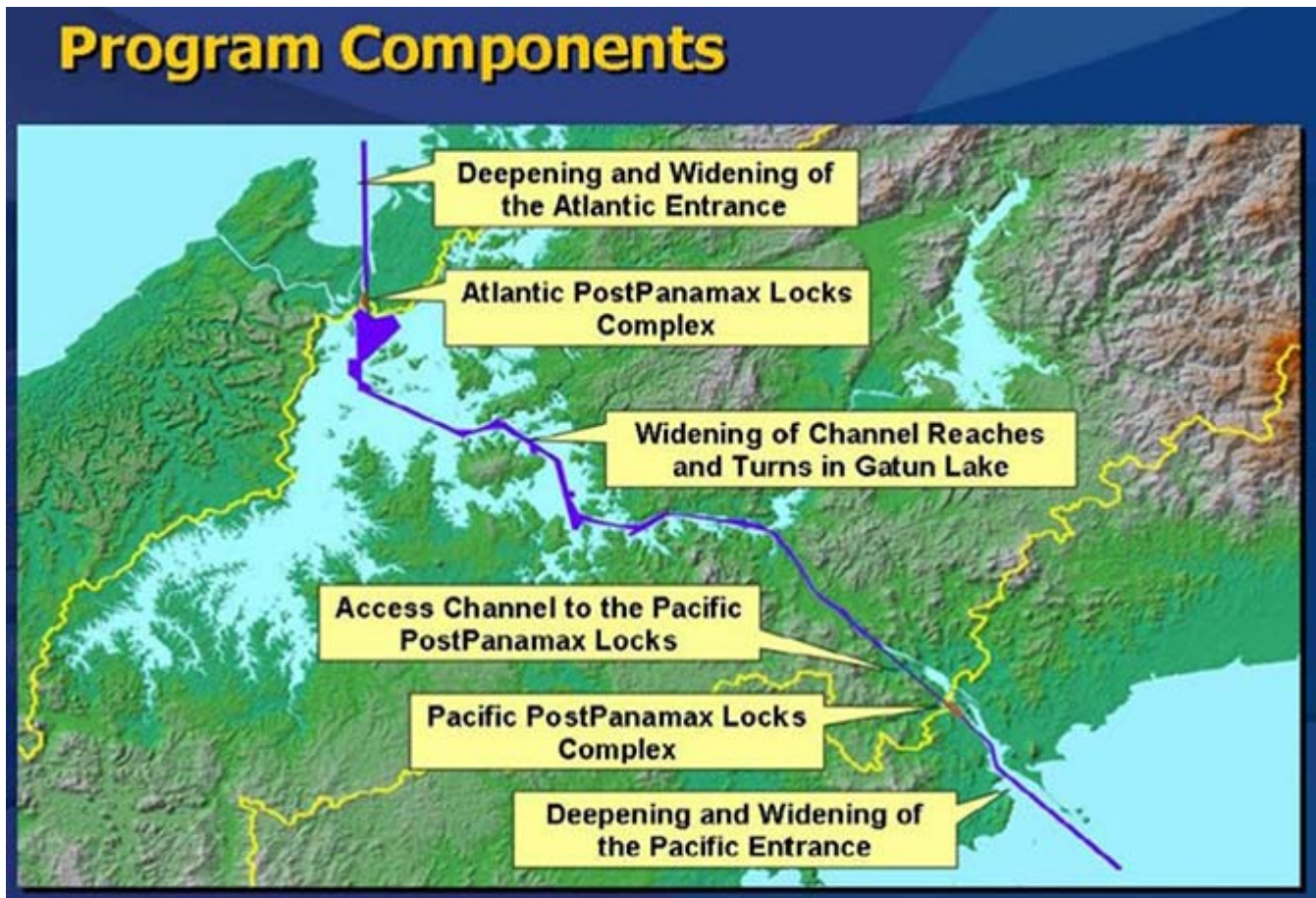
Components of Panama Canal Expansion Project
