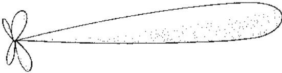
Figure 1303a. Freespace radiation pattern.
