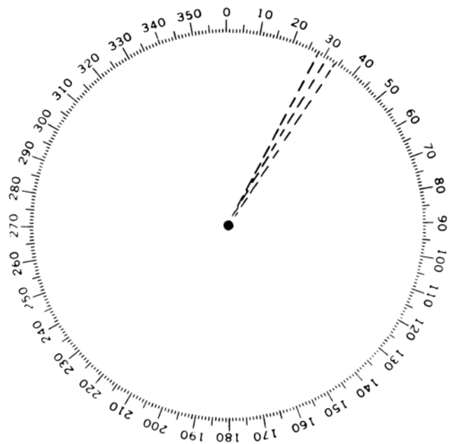
Figure 1308c. Ramark appears as broken radial line.
