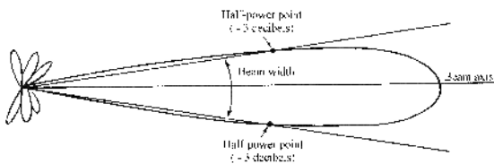
Figure 1303b. Radiation diagram.
